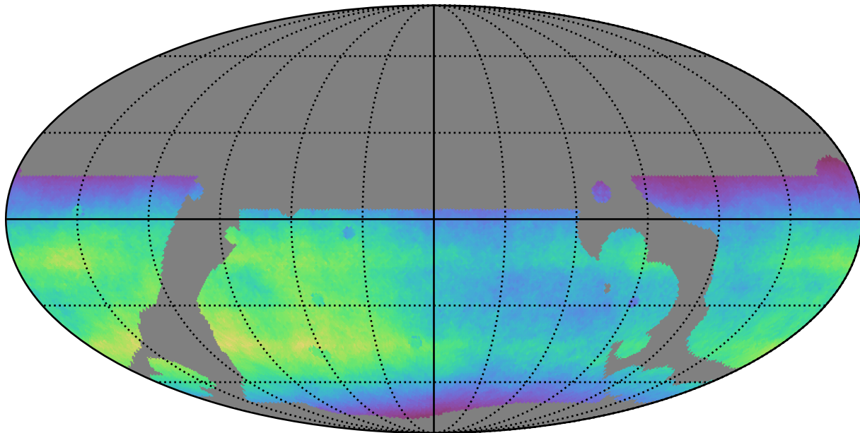
telescope_jerk_v3.5_10yrs WFD all bands: Normalized Teff
