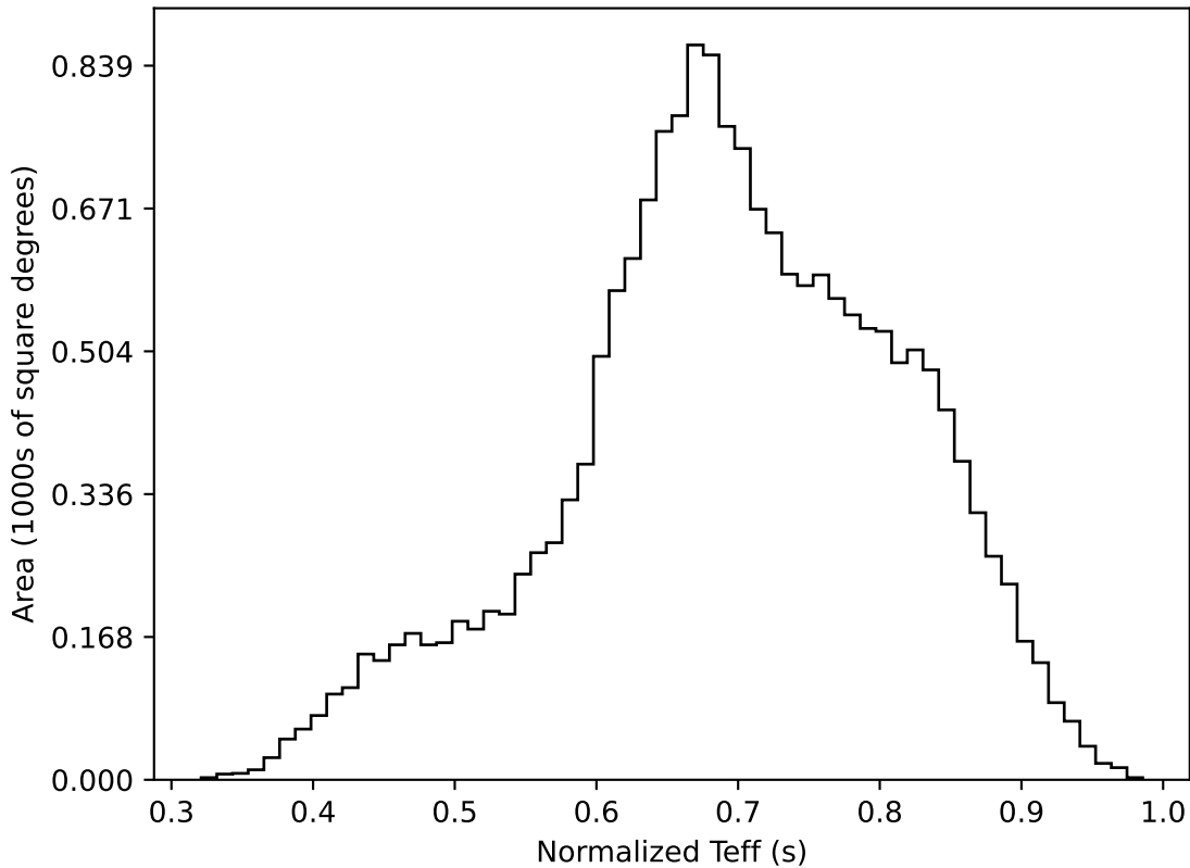
telescope_jerk_v3.5_10yrs WFD all bands: Normalized Teff
