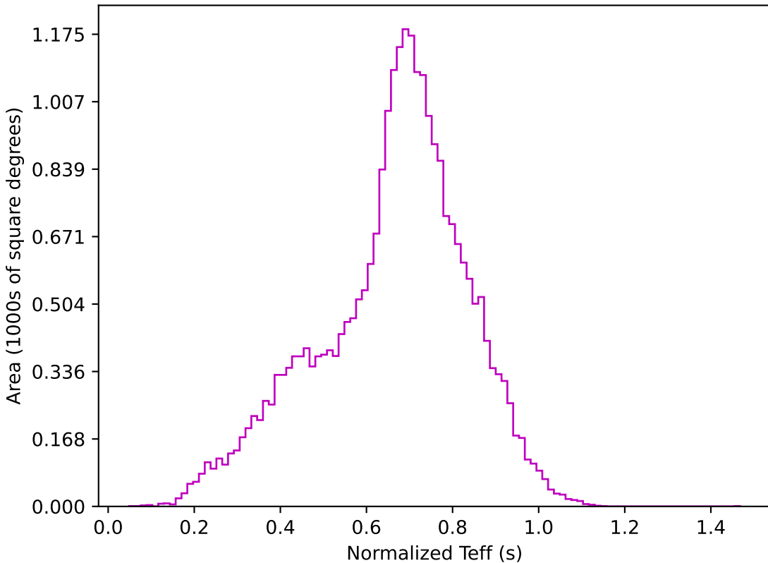
telescope_jerk_v3.5_10yrs All sky z band: Normalized Teff
