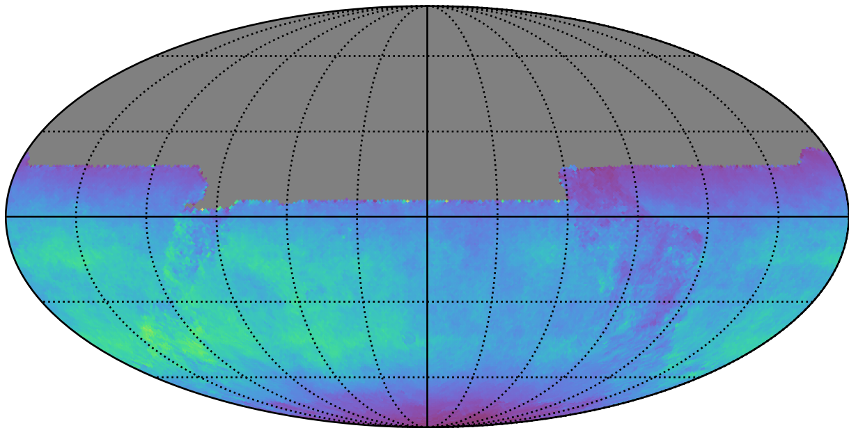
telescope_jerk_v3.5_10yrs All sky y band: Normalized Teff
