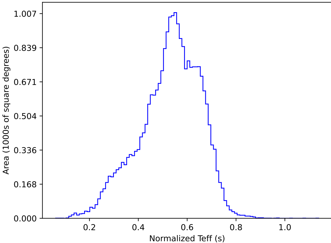
telescope_jerk_v3.5_10yrs All sky y band: Normalized Teff
