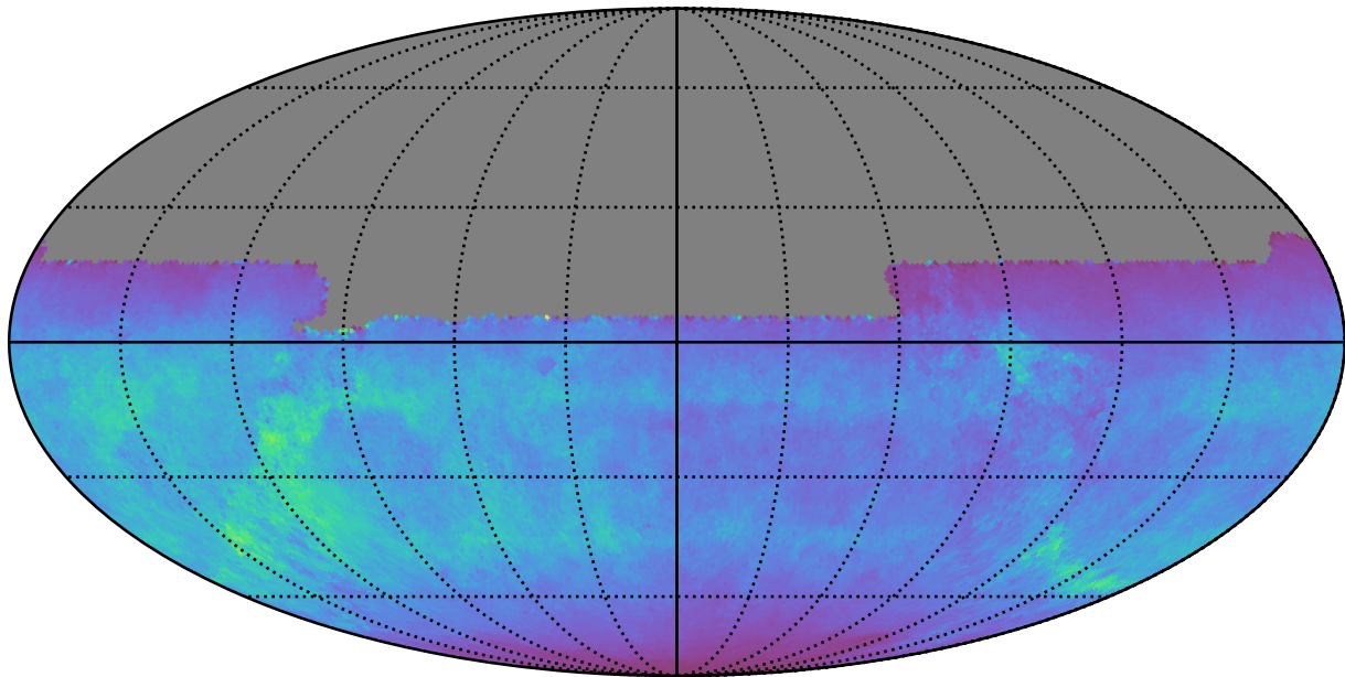
telescope_jerk_v3.5_10yrs All sky u band: Normalized Teff
