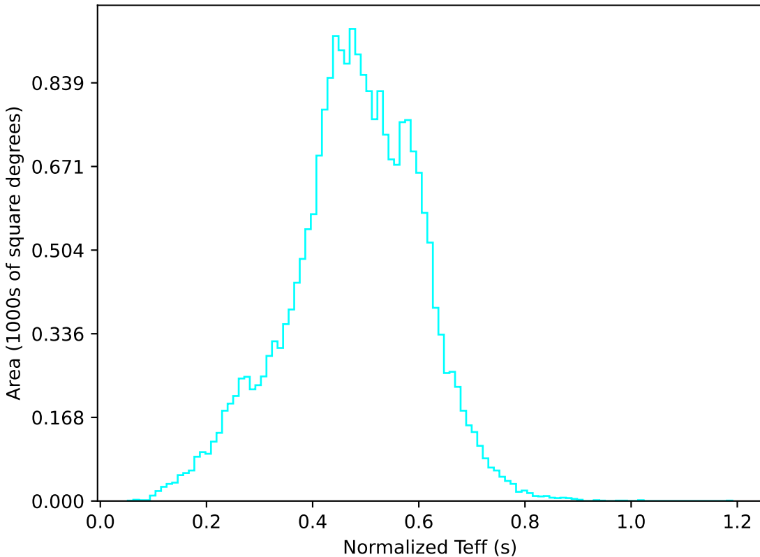
telescope_jerk_v3.5_10yrs All sky u band: Normalized Teff
