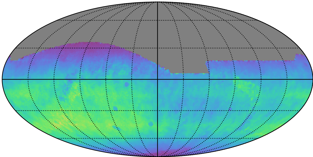
telescope_jerk_v3.5_10yrs All sky r band: Normalized Teff
