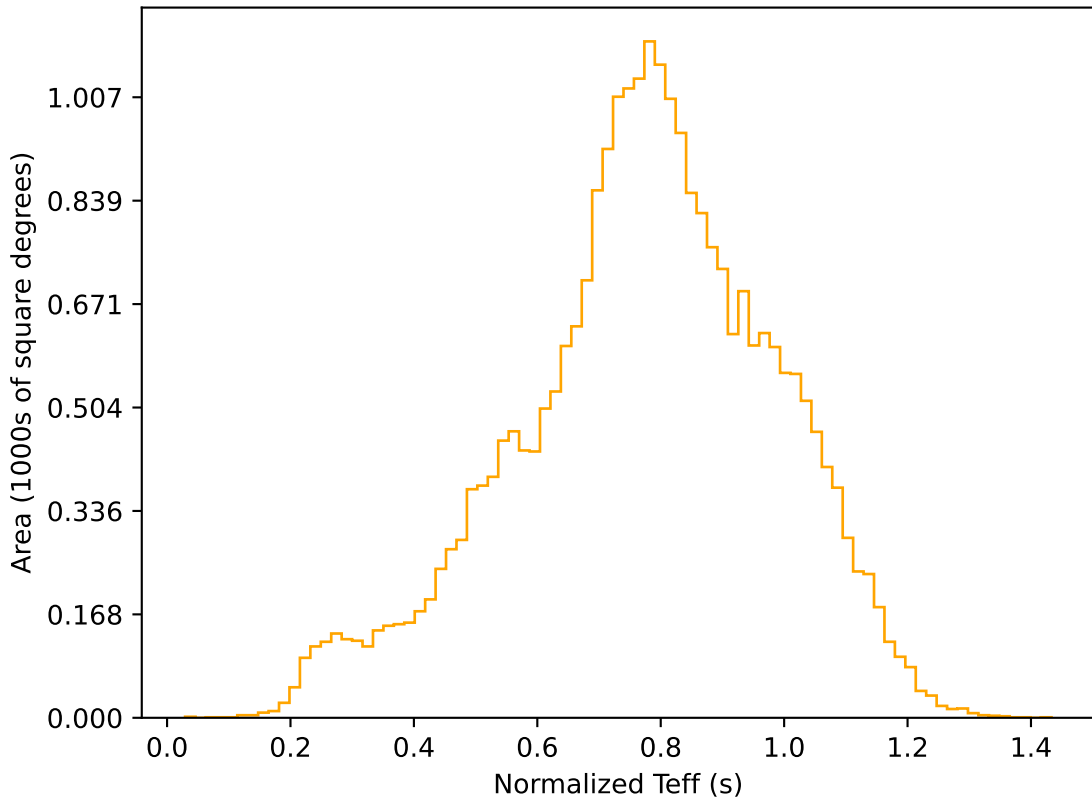
telescope_jerk_v3.5_10yrs All sky r band: Normalized Teff
