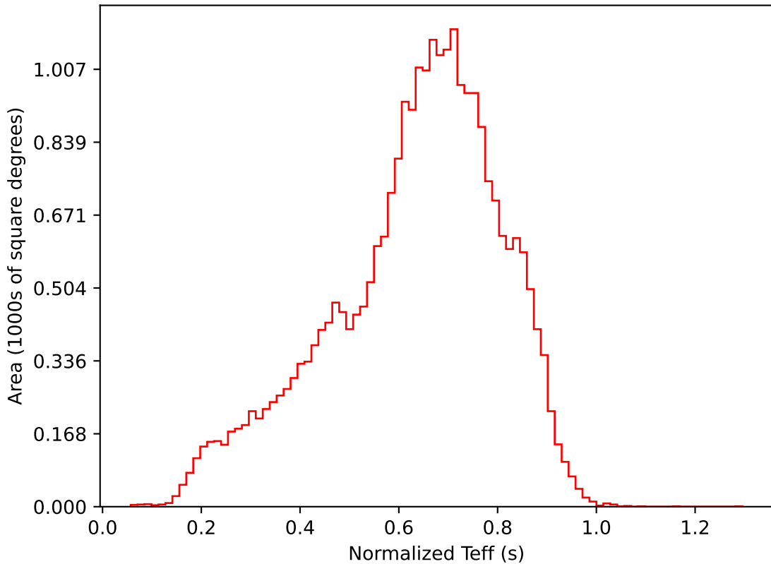
telescope_jerk_v3.5_10yrs All sky i band: Normalized Teff
