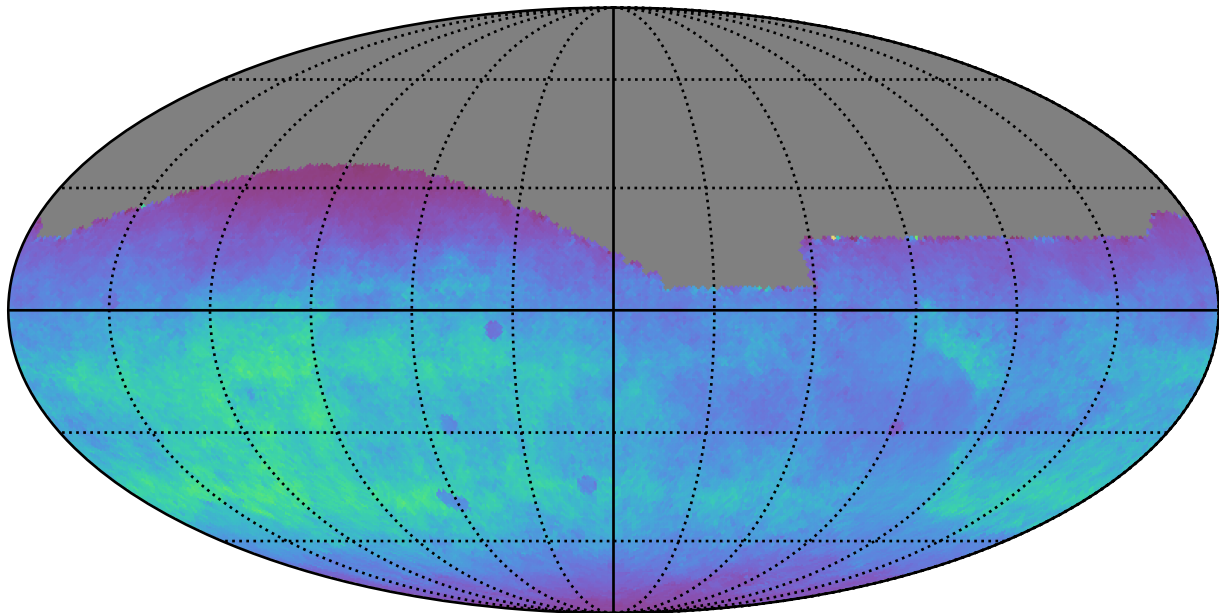
telescope_jerk_v3.5_10yrs All sky g band: Normalized Teff
