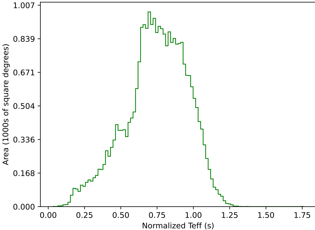
telescope_jerk_v3.5_10yrs All sky g band: Normalized Teff
