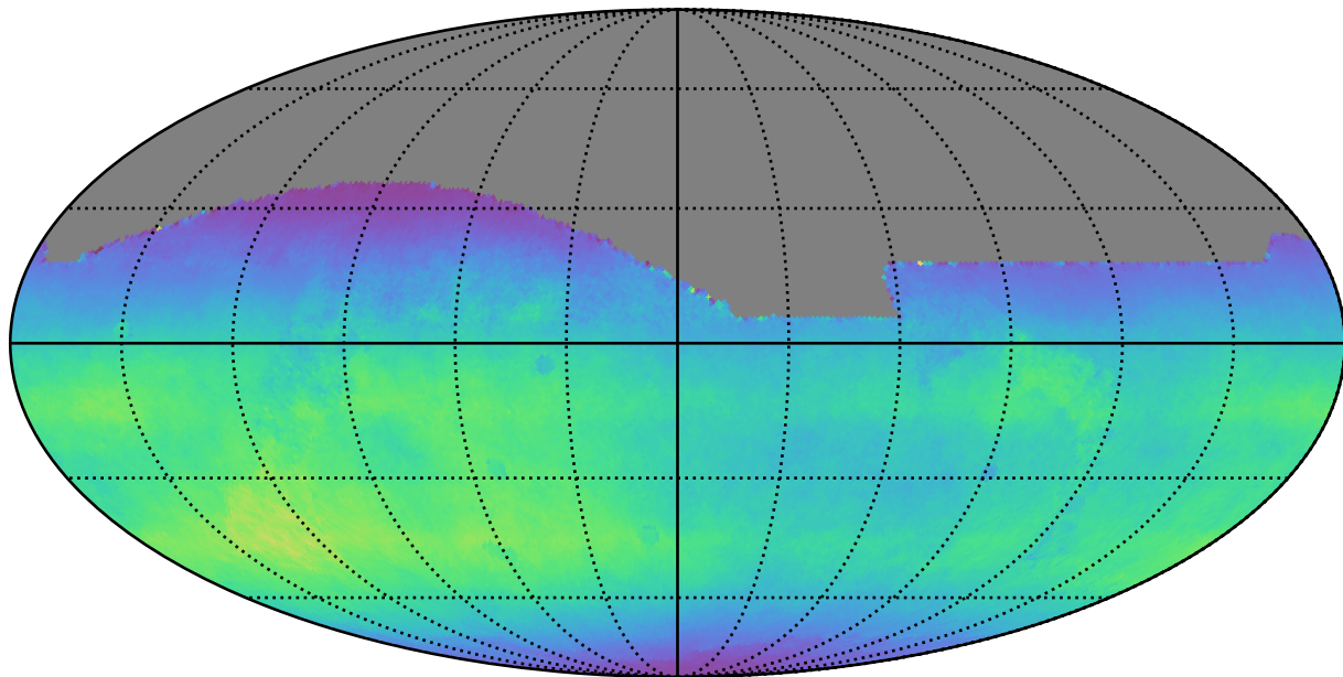
telescope_jerk_v3.5_10yrs All sky all bands: Normalized Teff
