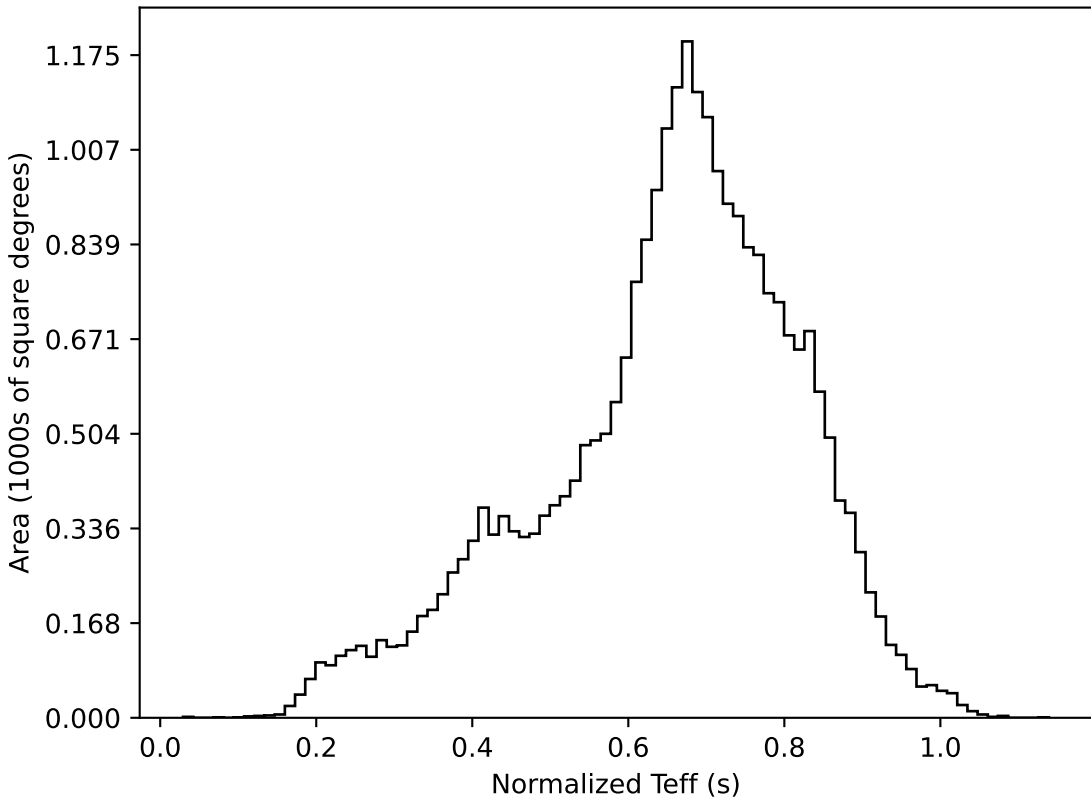
telescope_jerk_v3.5_10yrs All sky all bands: Normalized Teff
