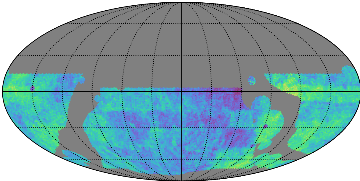
telescope_jerk_v3.5_10yrs WFD: Normalized Proper Motion Uncert @ 24.0
