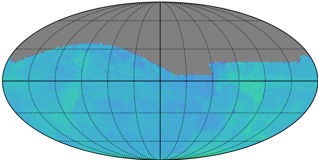
telescope_jerk_v3.5_10yrs All sky: Normalized Proper Motion Uncert @ 24.0
