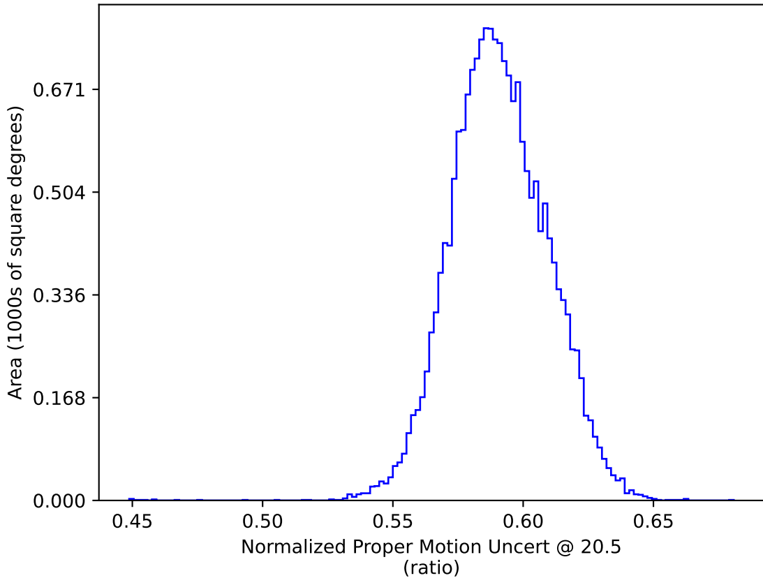
telescope_jerk_v3.5_10yrs WFD: Normalized Proper Motion Uncert @ 20.5
