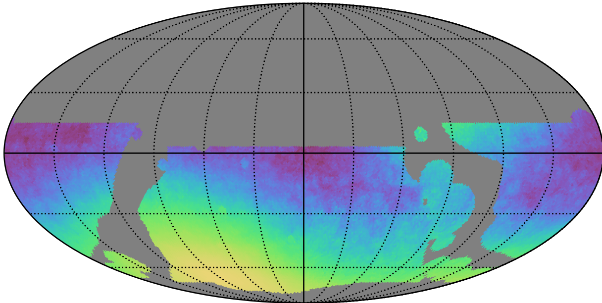
telescope_jerk_v3.5_10yrs WFD: Normalized Parallax Uncert @ 24.0
