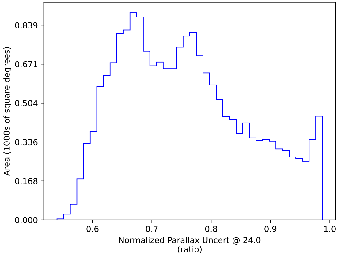
telescope_jerk_v3.5_10yrs WFD: Normalized Parallax Uncert @ 24.0
