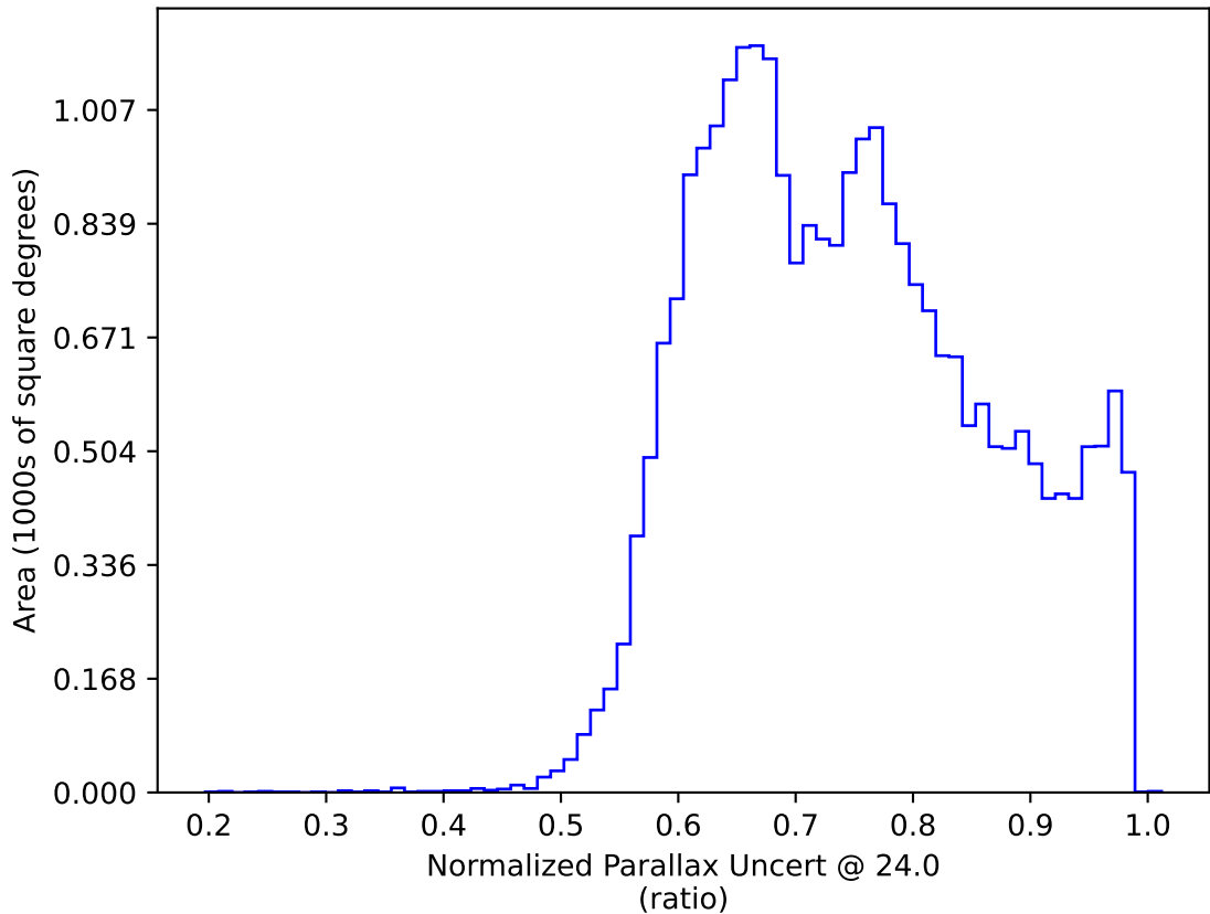
telescope_jerk_v3.5_10yrs All sky: Normalized Parallax Uncert @ 24.0
