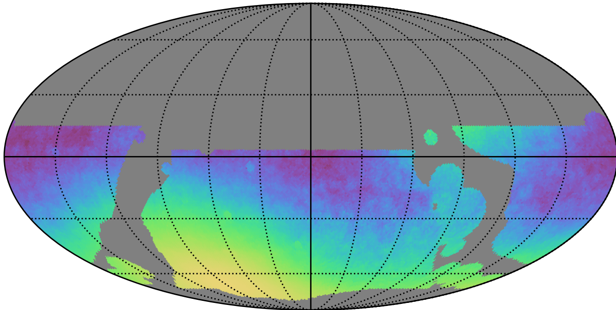
telescope_jerk_v3.5_10yrs WFD: Normalized Parallax Uncert @ 22.4
