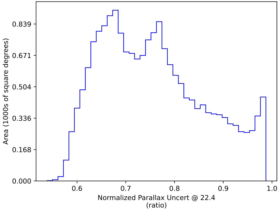
telescope_jerk_v3.5_10yrs WFD: Normalized Parallax Uncert @ 22.4
