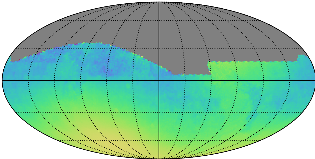
telescope_jerk_v3.5_10yrs All sky: Normalized Parallax Uncert @ 22.4
