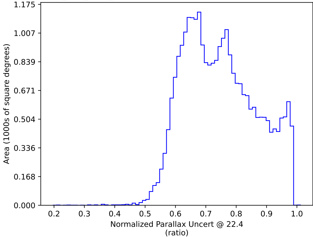
telescope_jerk_v3.5_10yrs All sky: Normalized Parallax Uncert @ 22.4
