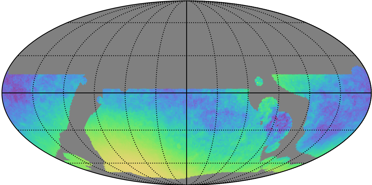
telescope_jerk_v3.5_10yrs WFD y band only: Normalized Parallax Uncert @ 21.3
