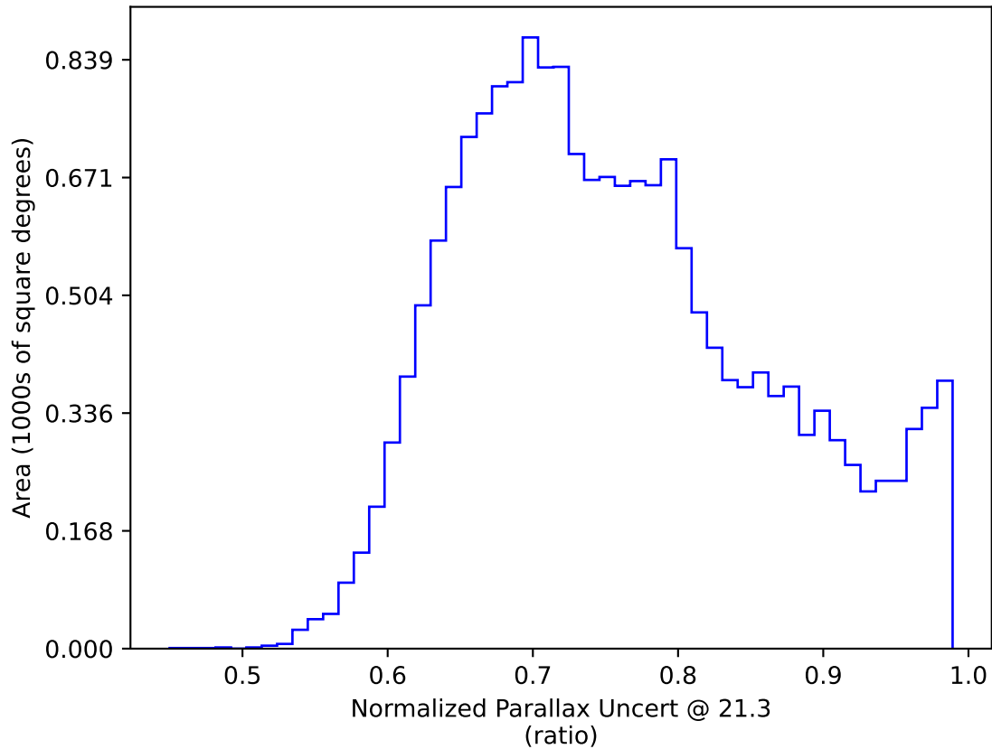
telescope_jerk_v3.5_10yrs WFD y band only: Normalized Parallax Uncert @ 21.3
