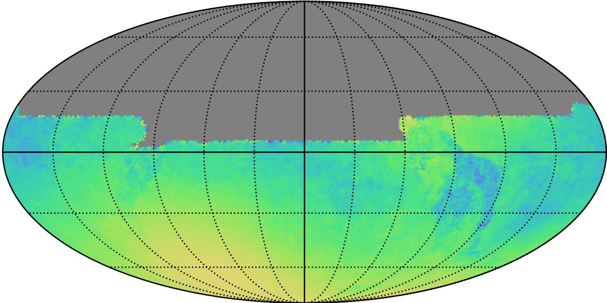
telescope_jerk_v3.5_10yrs All sky y band only: Normalized Parallax Uncert @ 21.3
