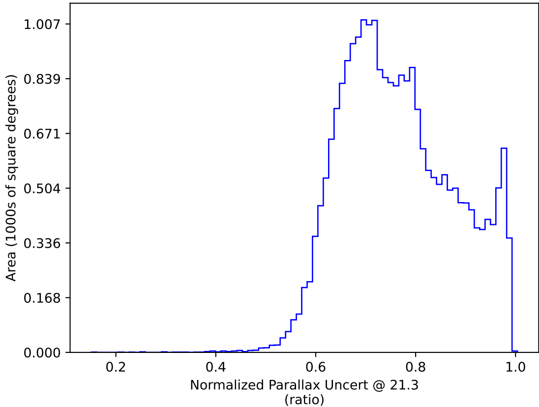
telescope_jerk_v3.5_10yrs All sky y band only: Normalized Parallax Uncert @ 21.3
