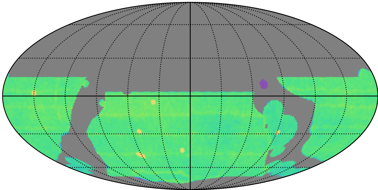
telescope_jerk_v3.5_10yrs WFD all bands: N Unique Nights
