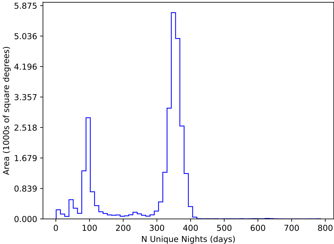
telescope_jerk_v3.5_10yrs All sky all bands: N Unique Nights
