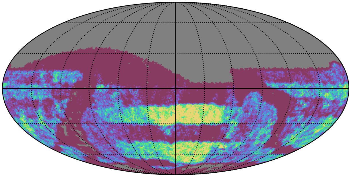
telescope_jerk_v3.5_10yrs Yr 3-4 z band: NVisits
