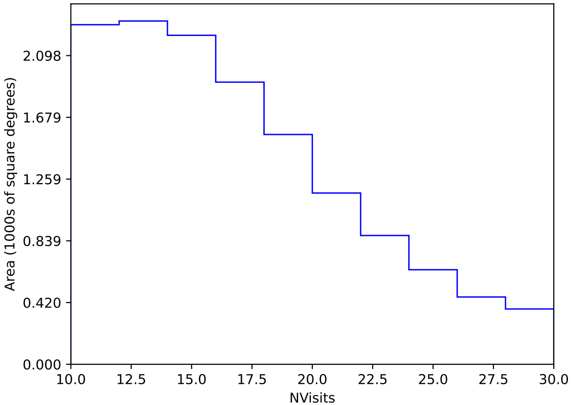
telescope_jerk_v3.5_10yrs Yr 3-4 y band: NVisits
