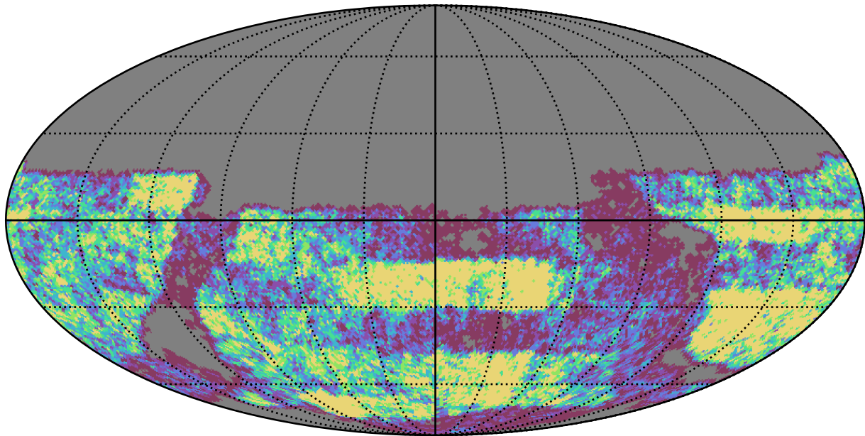
telescope_jerk_v3.5_10yrs Yr 3-4 u band: NVisits
