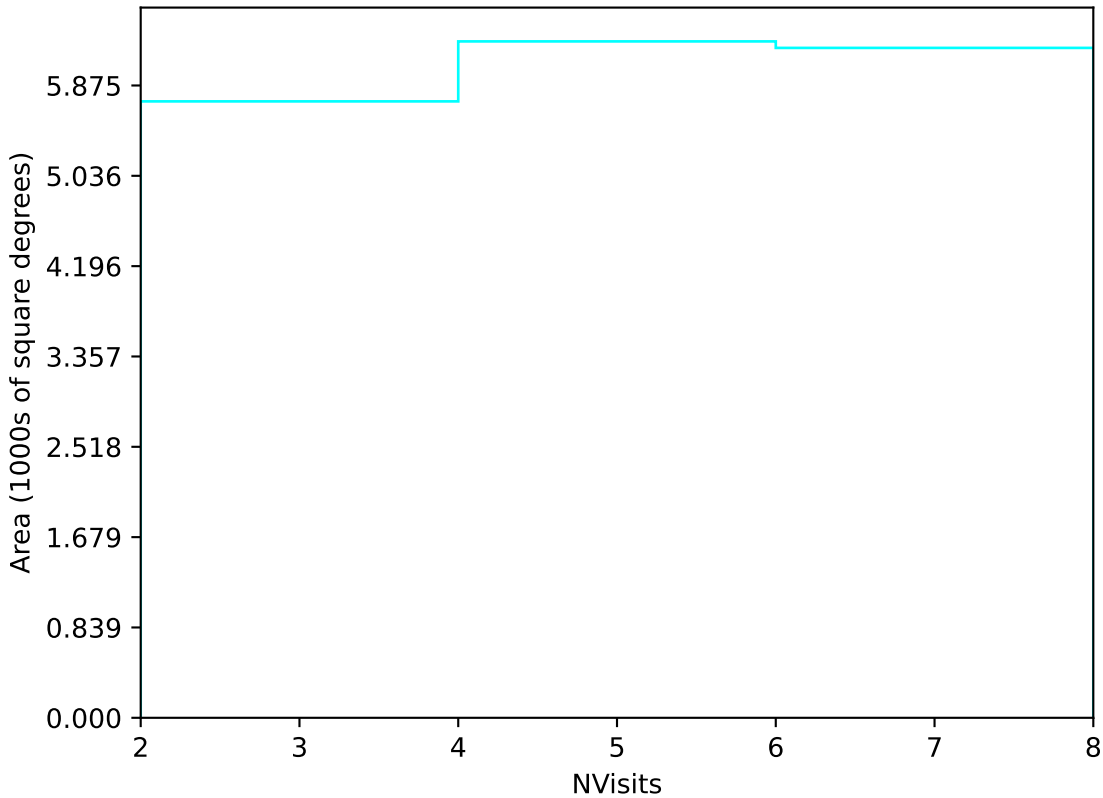
telescope_jerk_v3.5_10yrs Yr 3-4 u band: NVisits
