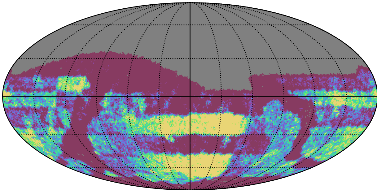
telescope_jerk_v3.5_10yrs Yr 3-4 r band: NVisits
