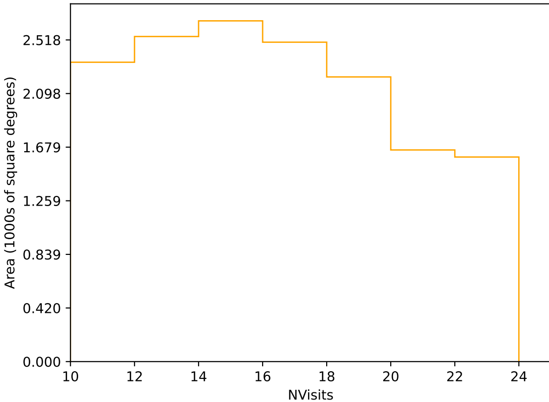
telescope_jerk_v3.5_10yrs Yr 3-4 r band: NVisits
