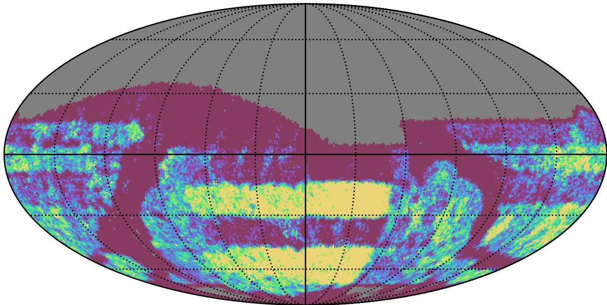
telescope_jerk_v3.5_10yrs Yr 3-4 i band: NVisits
