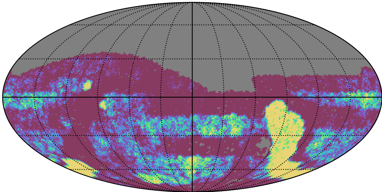
telescope_jerk_v3.5_10yrs Yr 3-4 g band: NVisits
