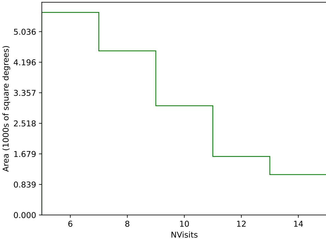
telescope_jerk_v3.5_10yrs Yr 3-4 g band: NVisits
