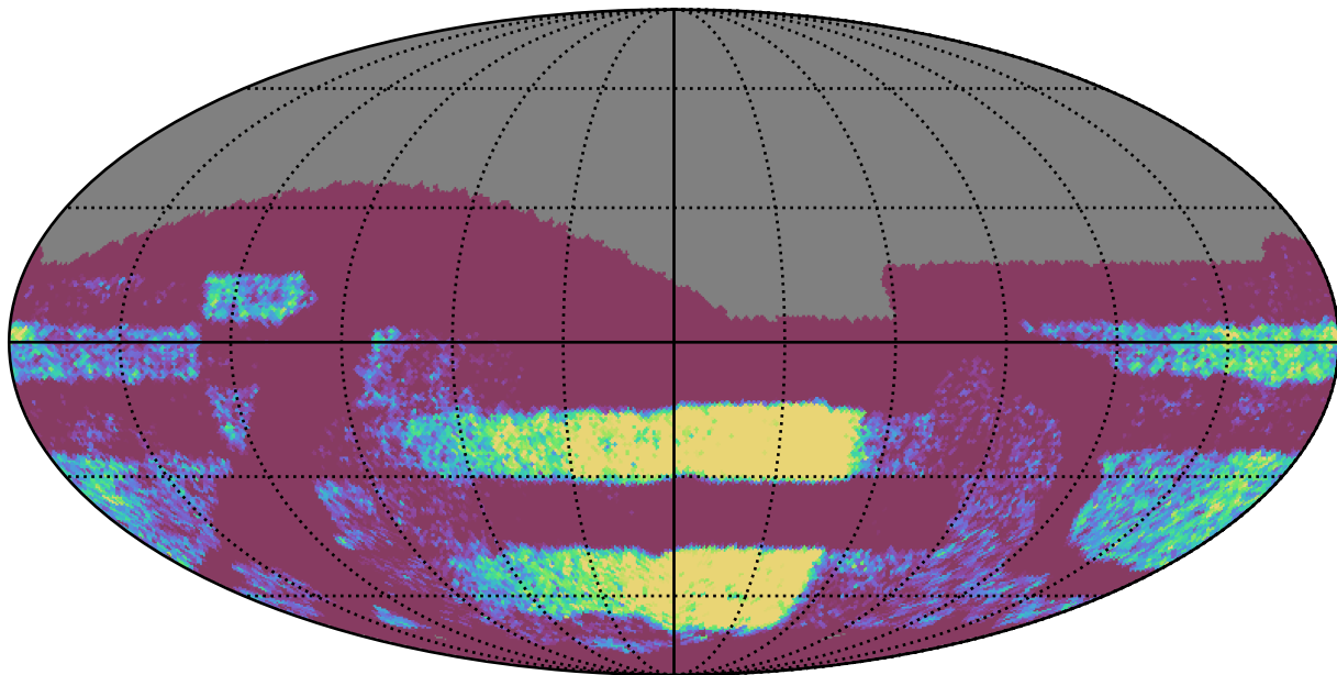
telescope_jerk_v3.5_10yrs Yr 3-4 all bands: NVisits
