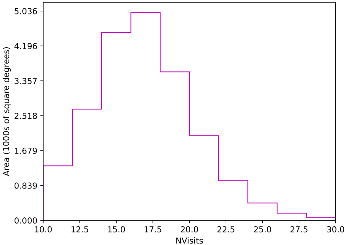
telescope_jerk_v3.5_10yrs Yr 1 z band: NVisits
