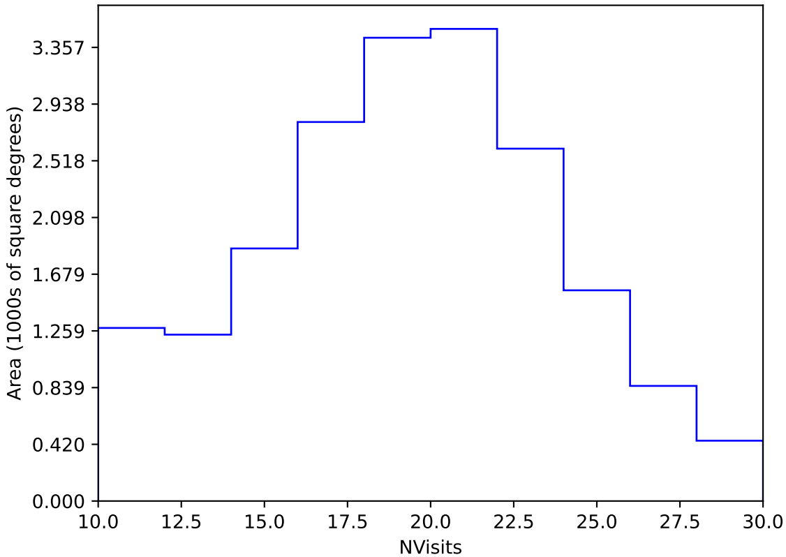
telescope_jerk_v3.5_10yrs Yr 1 y band: NVisits
