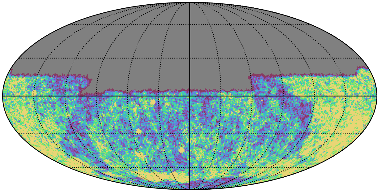
telescope_jerk_v3.5_10yrs Yr 1 u band: NVisits
