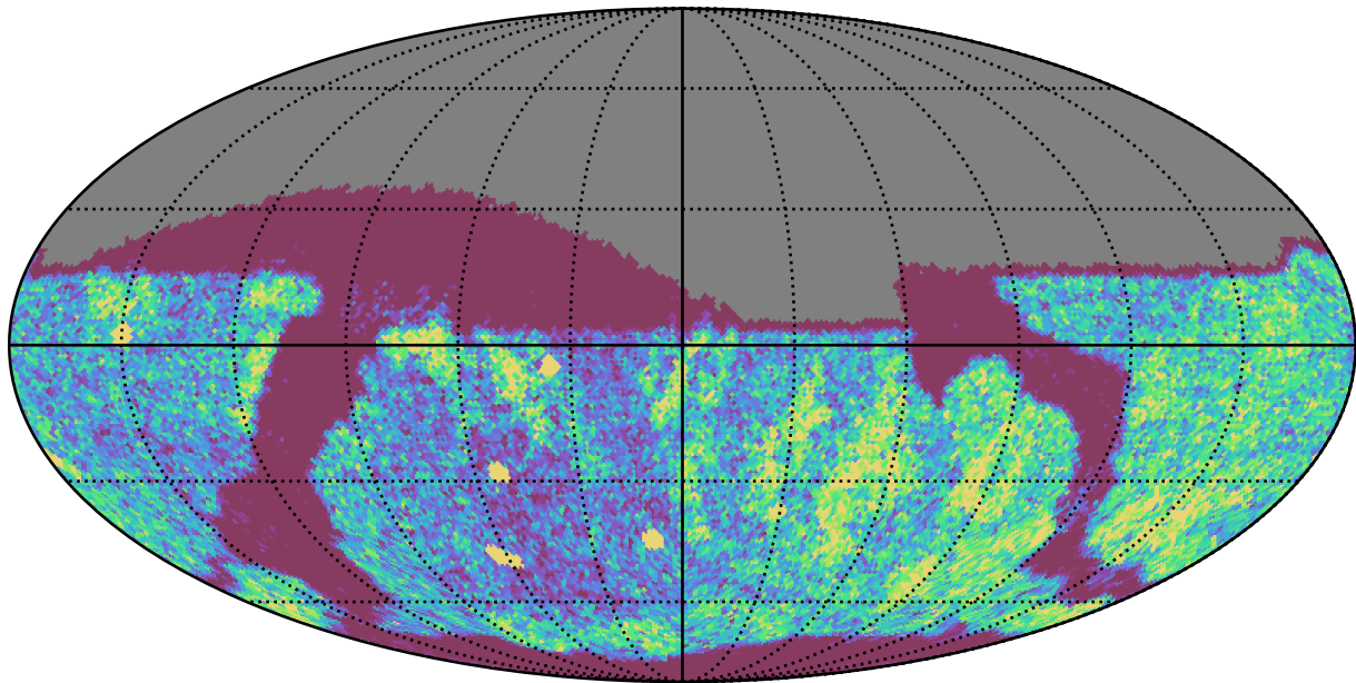
telescope_jerk_v3.5_10yrs Yr 1 r band: NVisits
