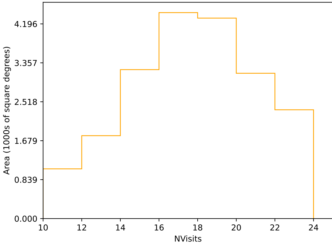
telescope_jerk_v3.5_10yrs Yr 1 r band: NVisits
