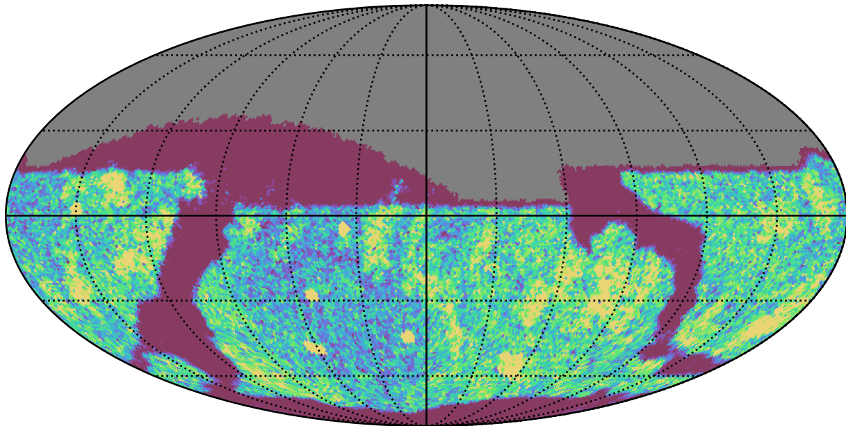
telescope_jerk_v3.5_10yrs Yr 1 i band: NVisits
