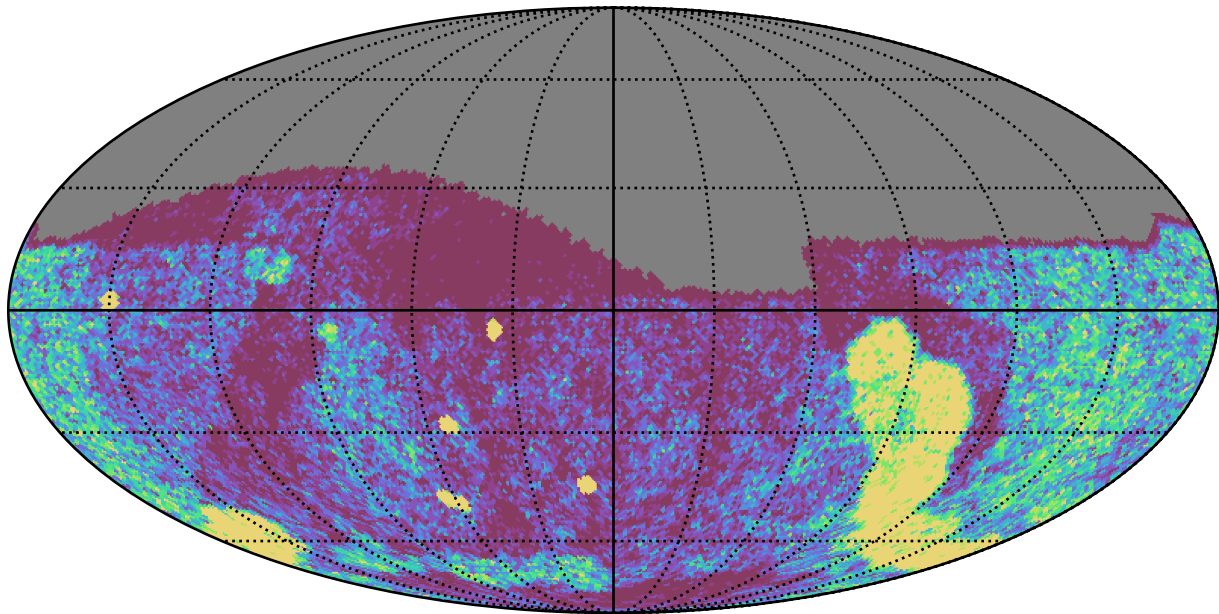
telescope_jerk_v3.5_10yrs Yr 1 g band: NVisits
