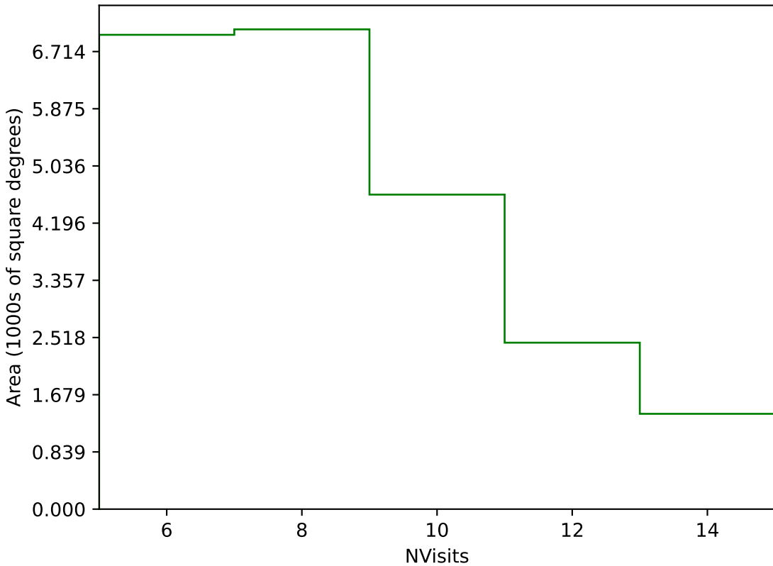
telescope_jerk_v3.5_10yrs Yr 1 g band: NVisits
