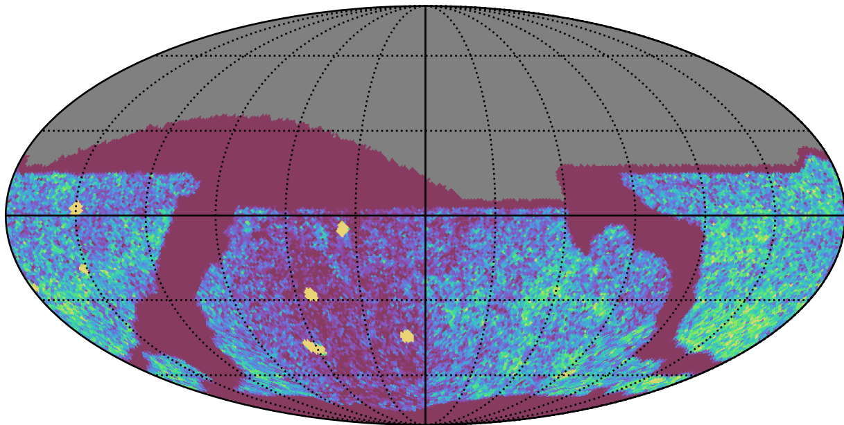
telescope_jerk_v3.5_10yrs Yr 1 all bands: NVisits
