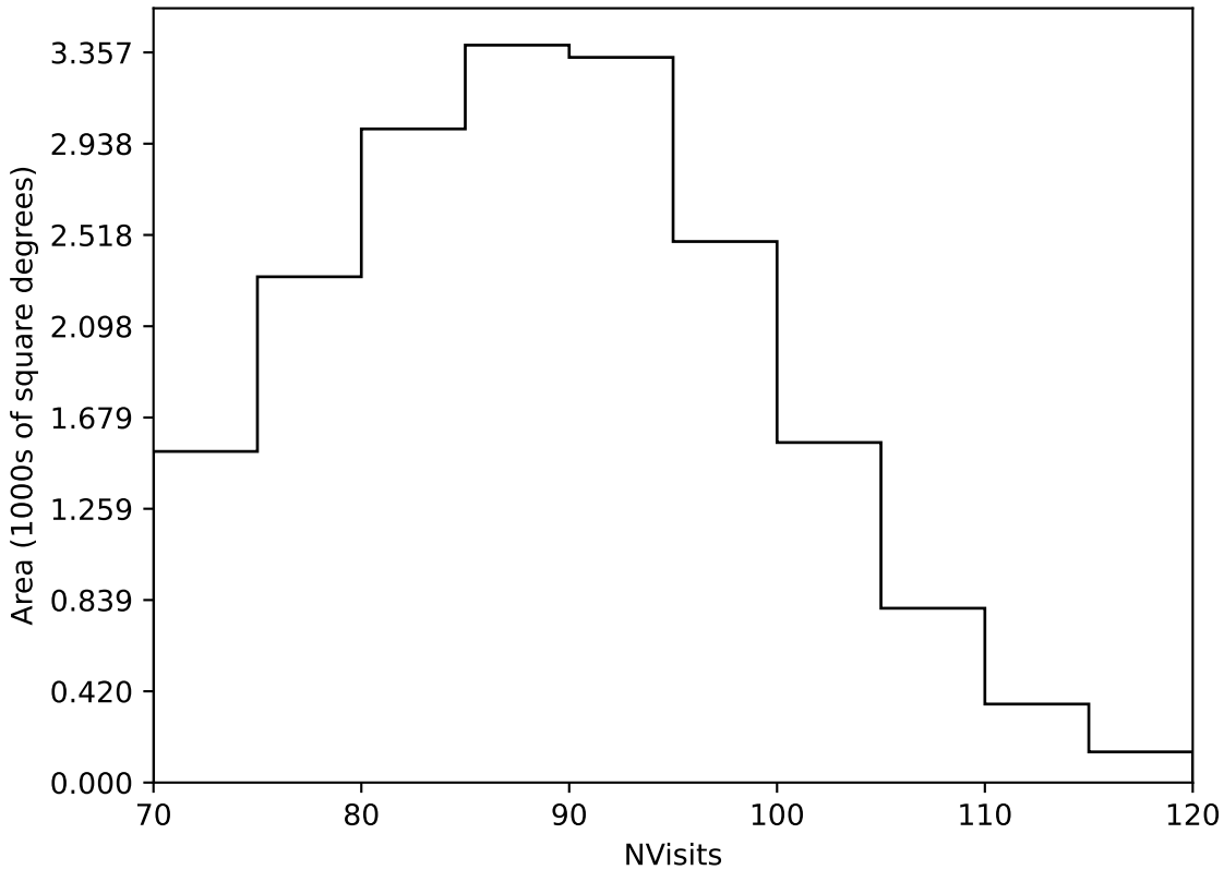
telescope_jerk_v3.5_10yrs Yr 1 all bands: NVisits
